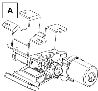
Driver Front Bracket Assembly
