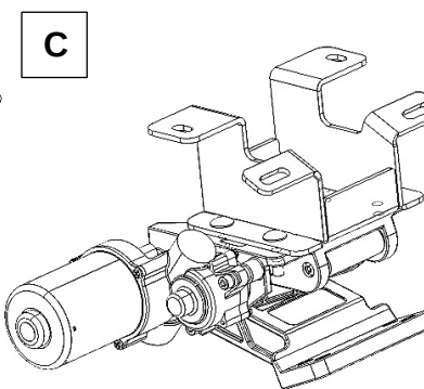
Passenger Front Bracket Assembly
