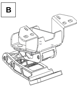
Driver Rear Bracket Assembly
